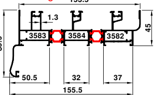
3585-3586 1.289 kg/m
