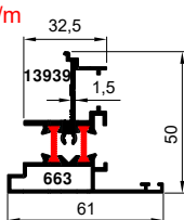
50-13939-663 1.191 kg/m
