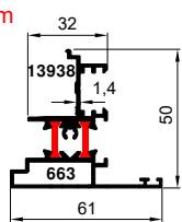
50-13938-663 1.166 kg/m
