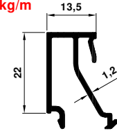
1949 0.306 kg/m
