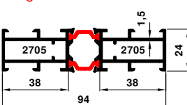
2705-2705 1.485 kg/m
