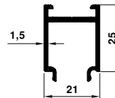
11617 0.359 kg/m
