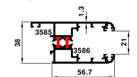
3585-3586 1.289 kg/m
