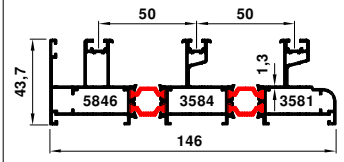
5846-3584-3581 2.713 kg/m
