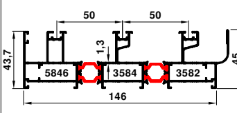
5846-3584-3582 2.866 kg/m
